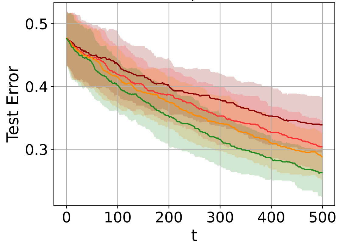
N = 10 particles
